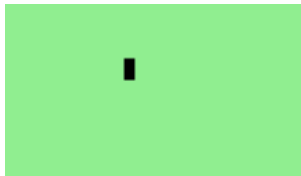
Figure 10.20.: Snake
