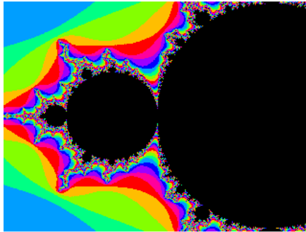
Figure 11.35: Fractals: Mandelbrot set
