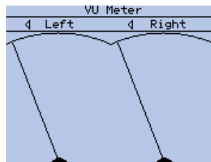
Figure 11.42.: VU-Meter
