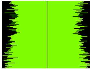
Figure 11.37.: Oscilloscope
