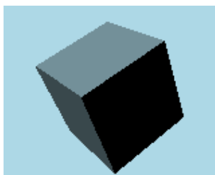
Figure 11.30.: Cube
