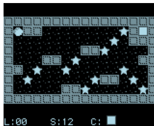
Figure 11.25.: Star game
