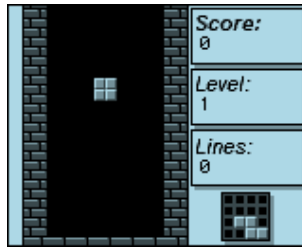
Figure 11.18.: Rockblox
