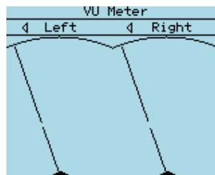
Figure 11.40.: VU-Meter
