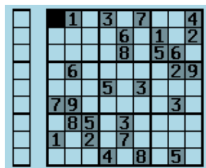
Figure 11.26.: Sudoku
