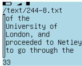
Figure 11.42.: Text Viewer
