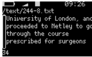
Figure 12.43.: Text Viewer
