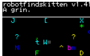
Figure 12.18.: Robotfindskitten
