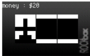
Figure 12.11.: Jackpot
