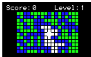
Figure 12.5.: Clix
