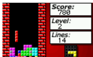
Figure 12.19.: Rockblox
