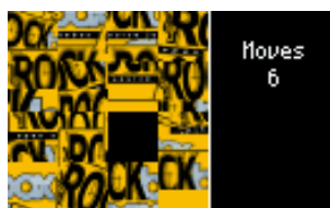
Figure 12.20.: Sliding puzzle
