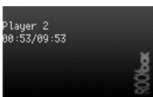
Figure 12.49.: Chess Clock
