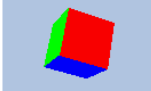
Figure 12.31.: Cube
