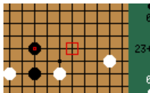
Figure 12.9.: Goban
