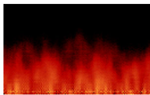
Figure 12.33.: Fire
