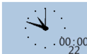
Figure 12.50.: Clock
