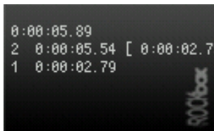
Figure 12.54.: Stopwatch
