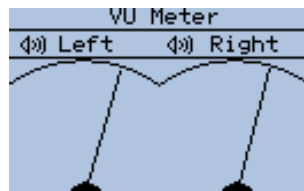
Figure 12.41.: VU-Meter
