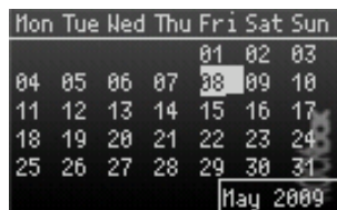
Figure 12.48.: Calendar
