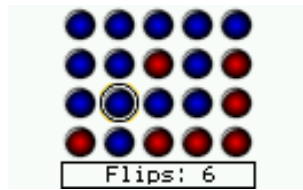
Figure 12.8.: Flipit
