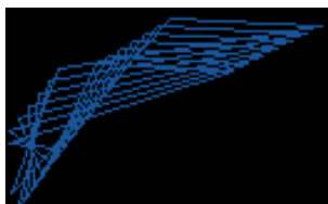
Figure 12.32.: Demystify
